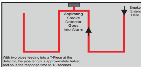
Figure 2. Two Sampling Pipe
