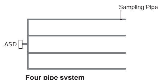
Figure 3. Multiple pipe configurations for an ASD sampling pipe network
