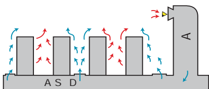
A targeted supply air supply with a hot return air system. Cold supply air mixes with hot return air. Install air sampling ports at main return into HVAC/CRAC unit.
