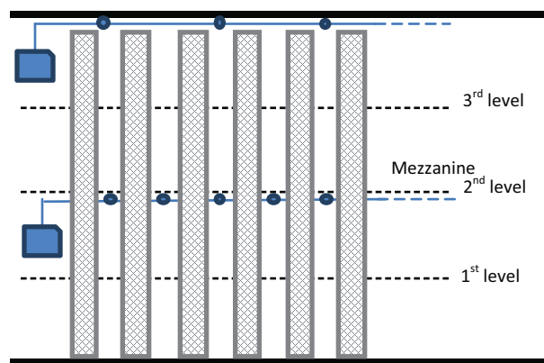
Figure 21. – Example of Multi-Level Detection (Ceiling and Intermediate Level)
