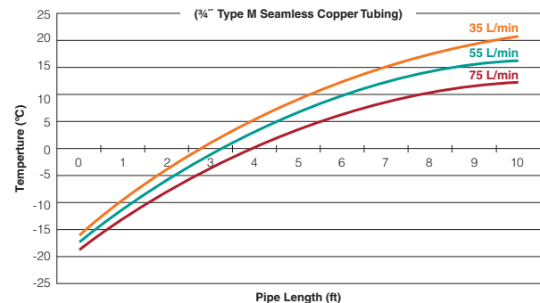
Figure 6. Distances needed to heat air in sampling pipe
