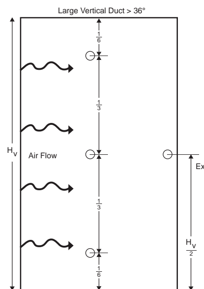
Figure 4. Large vertical ducts
