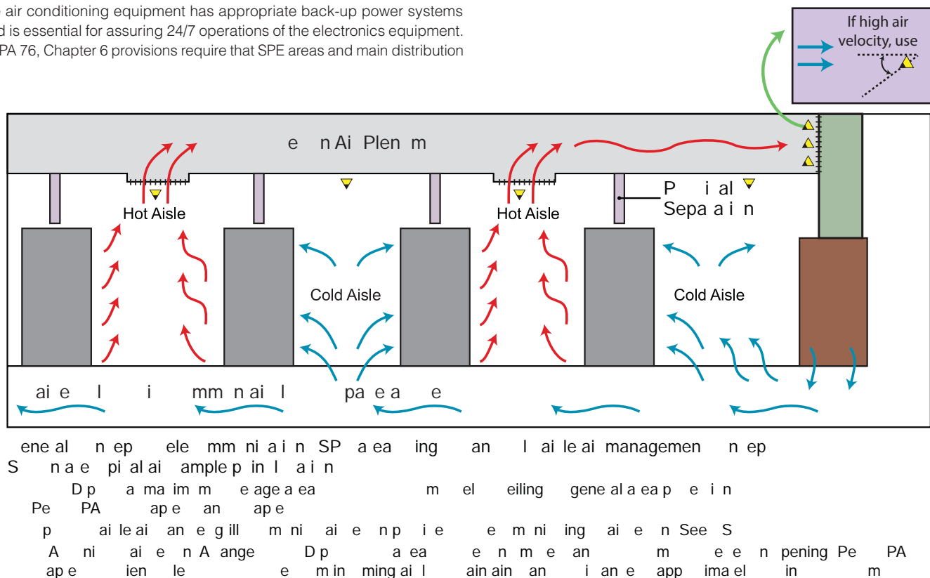
Figure 8. – Example of air sampling port locations in a Signal Processing Equipment (SPE) Area
